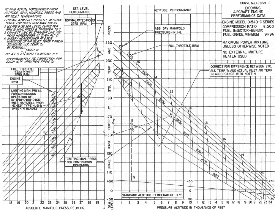
Figure 3-17. Sea Level and Altitude Performance Curve - IO-540-C
